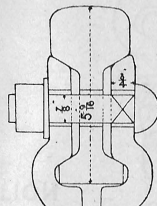
SECTION OF RAIL & FISH PLATES FIG 6
