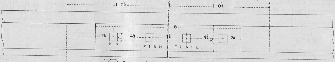
Bolt hole thro rail
