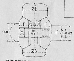
SECTION OF RAIL & FISH PLATES FIG 6
