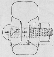
SECTION OF RAIL & FISH PLATES FIG 6
