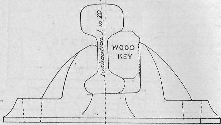
SECTION FIG 3
