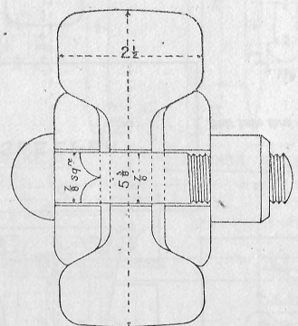
SECTION OF RAIL & FISH PLATES
