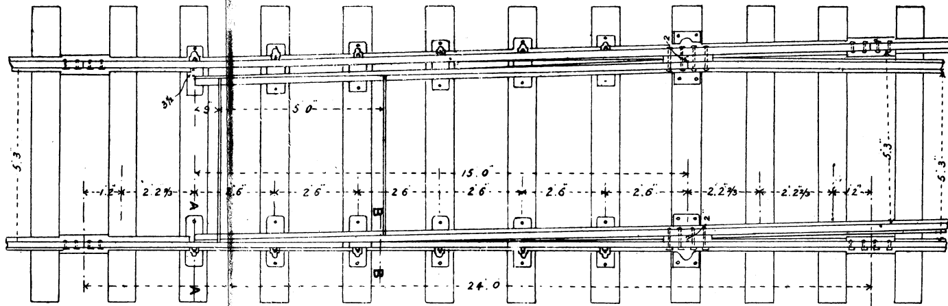
Fig 1 15'0" POINTS AND STOCK RAILS
