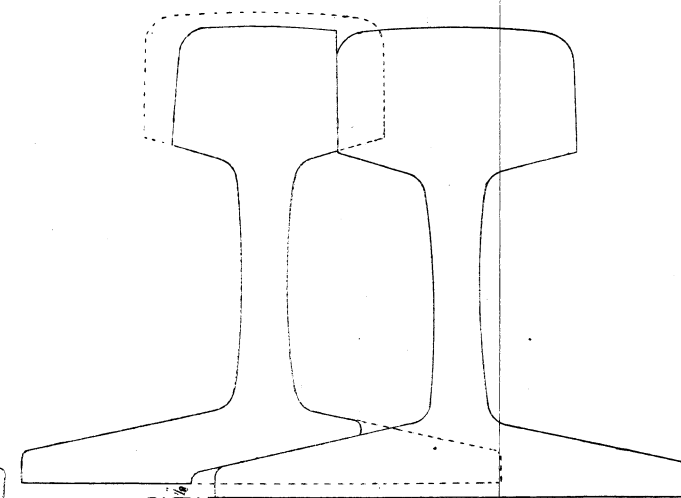
— Fig 5 — — SECTION AT EF —
