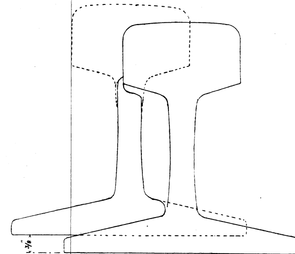
— Fig 2 — — SECTION AT AB — — TOE OF POINTS —
