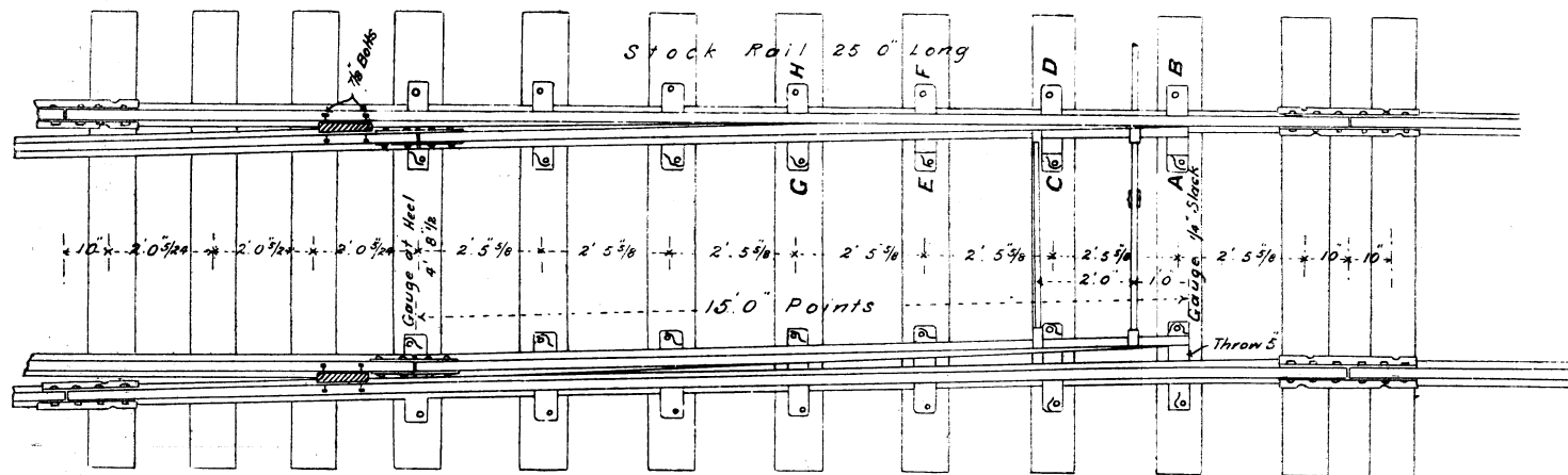
— Fig 1 — — 15.0 POINTS AND STOCK RAILS —
