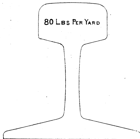
— Fig 3 — — RAIL HALF SIZE —
