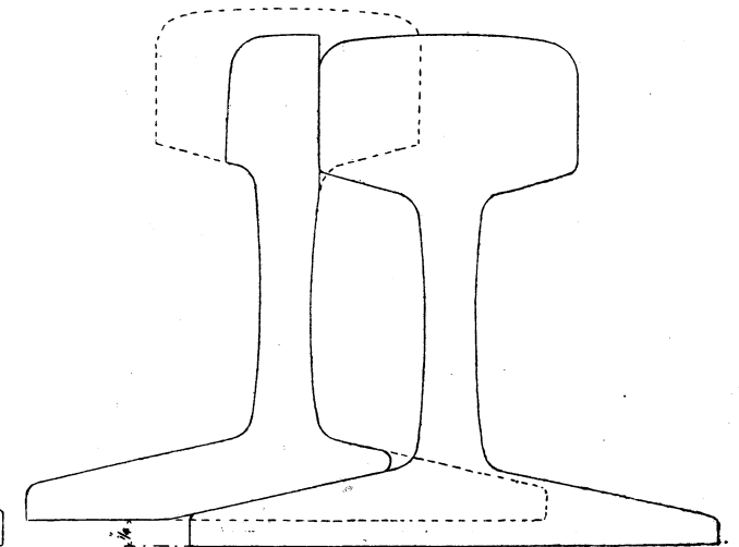
— Fig 6 — — SECTION AT CD —
