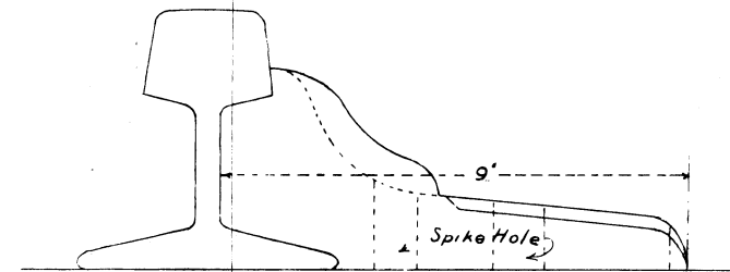
Fig 6 ELEVATION OF SUPPORT
