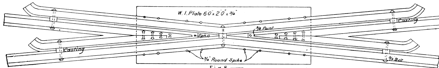
Fig 5 DIAMOND CROSSING 1 IN 5 1/4
