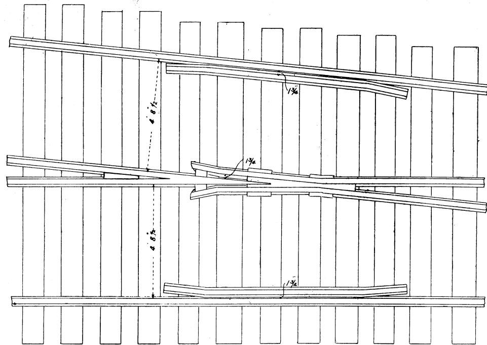
Fig 1 CROSSING 1 IN 10
