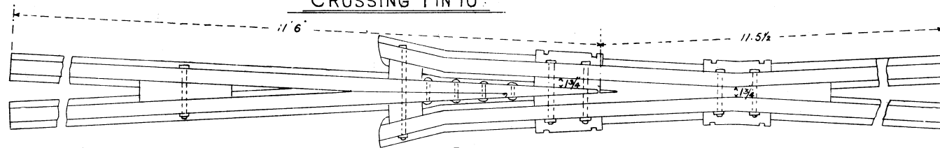
Fig 3 CROSSING 1 IN 10
