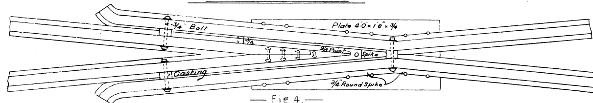
Fig 4 CROSSING 1 IN 5 1/4
