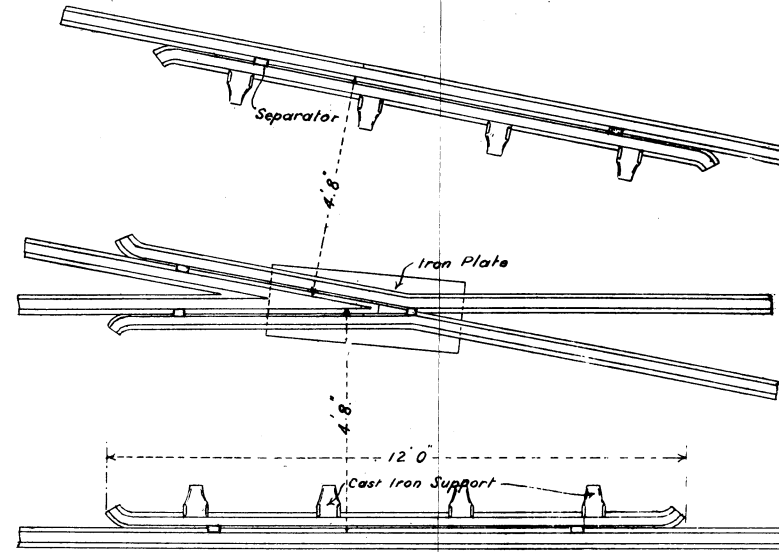
Fig 2 CROSSING 1 IN 5 1/4
