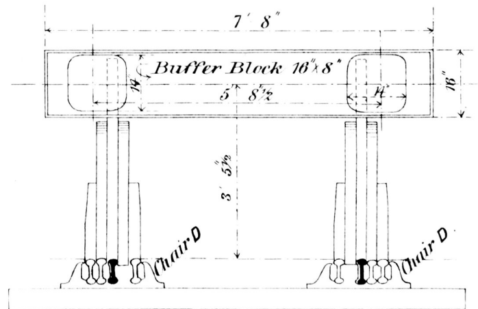
END ELEVATION.
