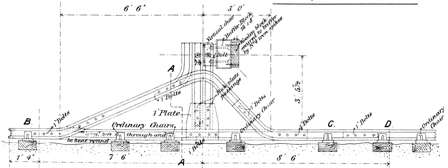
ELEVATION.
