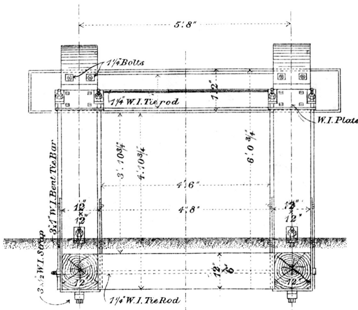
ELEVATION (BACK)
