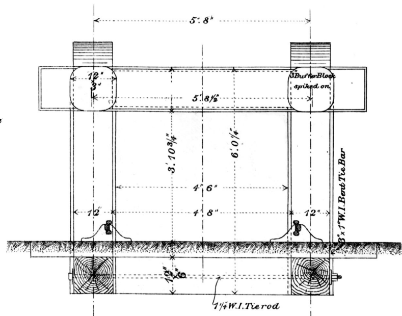
ELEVATION (FRONT)
