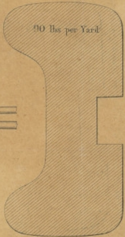
Section of Rail full size as rolled for the Great Northern Railway Comp y
