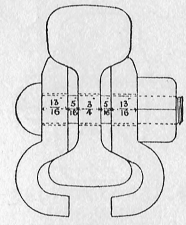
SECTION OF RAIL & FISH PLATES FIG 5.
