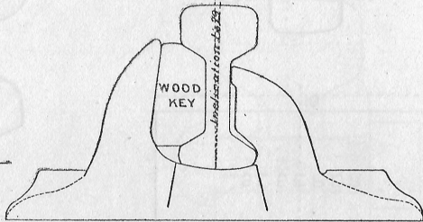
SECTION OF RAIL FIG 1.
