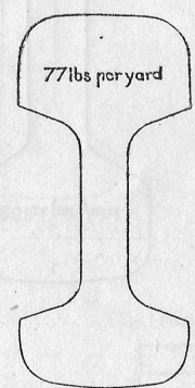
SECTIONS OF RAILS FIG 1
