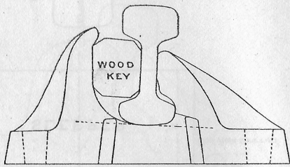
SECTION FIG 3.
