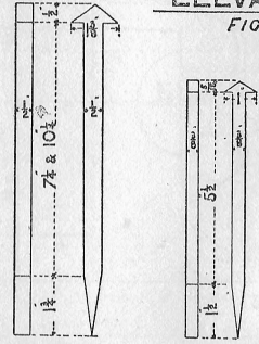
ANCHOR HEAD SPIKES
