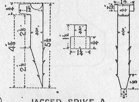
JAGGED SPIKE A
