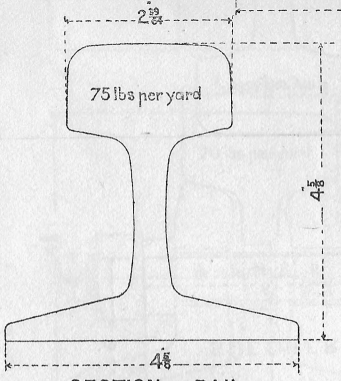
SECTION OF RAIL FIG 1.
