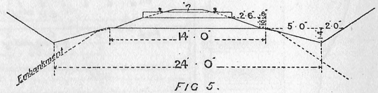
FIG 5. Section of fine Gravel Ballast & for Cementing Gravel
