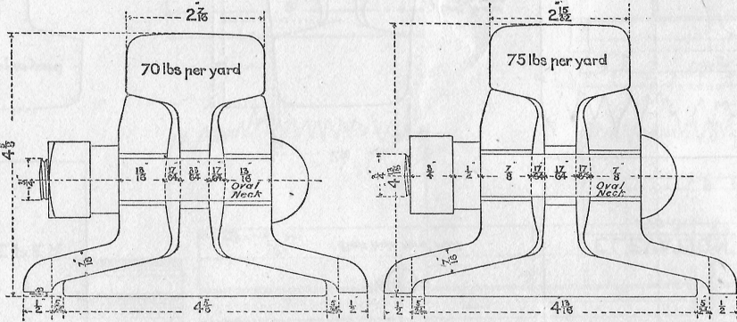
SECTION OF RAIL & FISH PLATES
