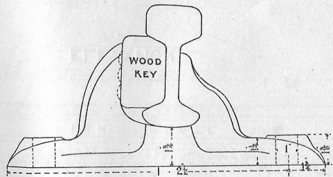
SECTION FIG 5.
