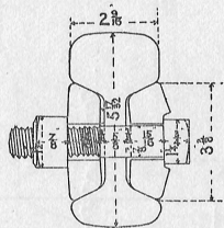
SECTION OF RAIL & FISH PLATES FIG 3.
