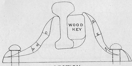
SECTION FIG 4
