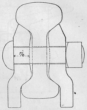
SECTION OF RAIL & FISH PLATES FIG 2
