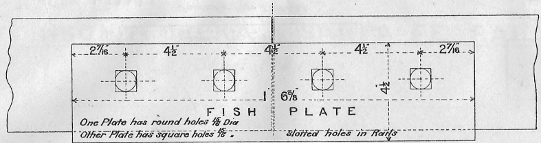
ELEVATION FIG 3
