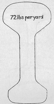
SECTION OF RAIL FIG 1
