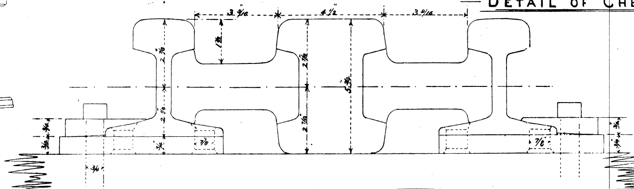
— Fig 3 — — SECTION D.D. —
