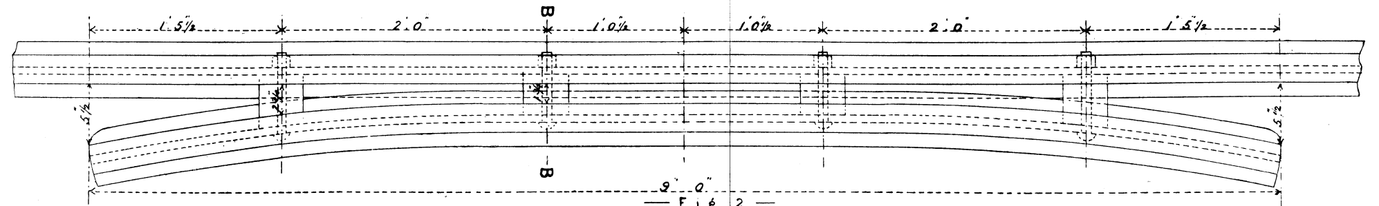
— Fig 2 — — DETAIL OF CHECK RAIL —
