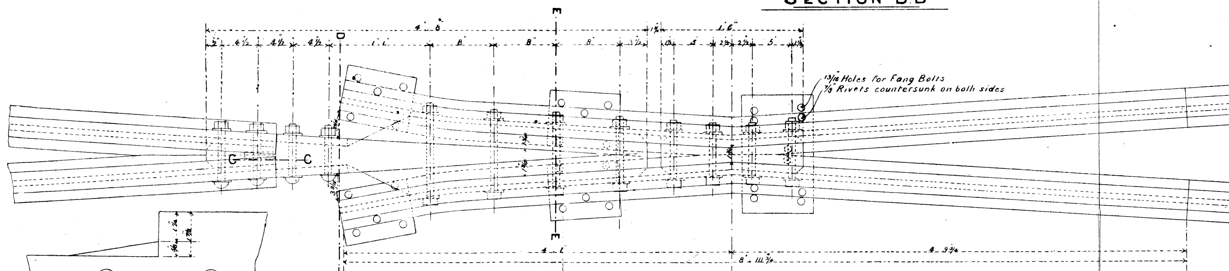
— Fig 5 — — DETAIL OF CROSSING 1 IN 8 —
