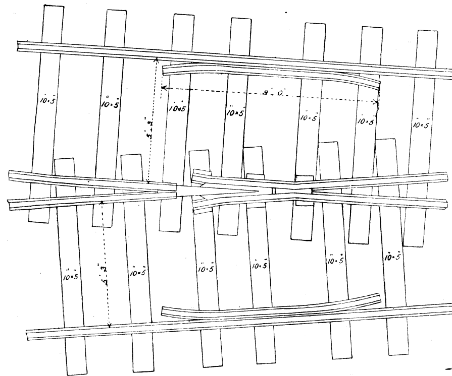
— Fig 1 — — CROSSING 1 IN 8. —
