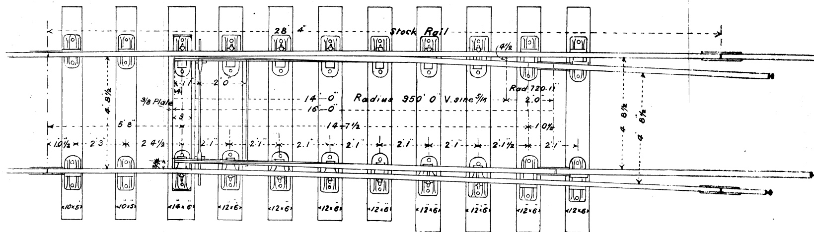
Fig 1 14.0 POINTS AND STOCK RAIL
