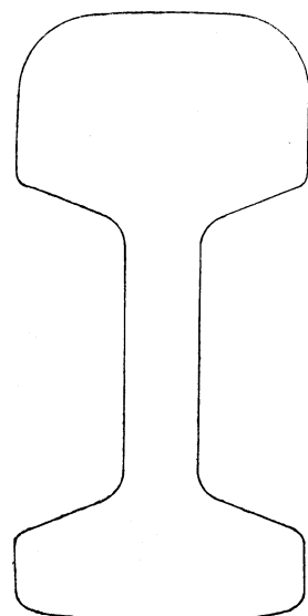
Fig 2 SECTION OF RAIL HALF SIZE
