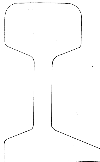
Inclination of 1 in 20 Fig 3 SECTION OF POINT BLADE RAIL HALF SIZE
