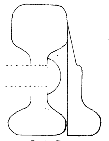
SECTION AT TOE OF POINTS
