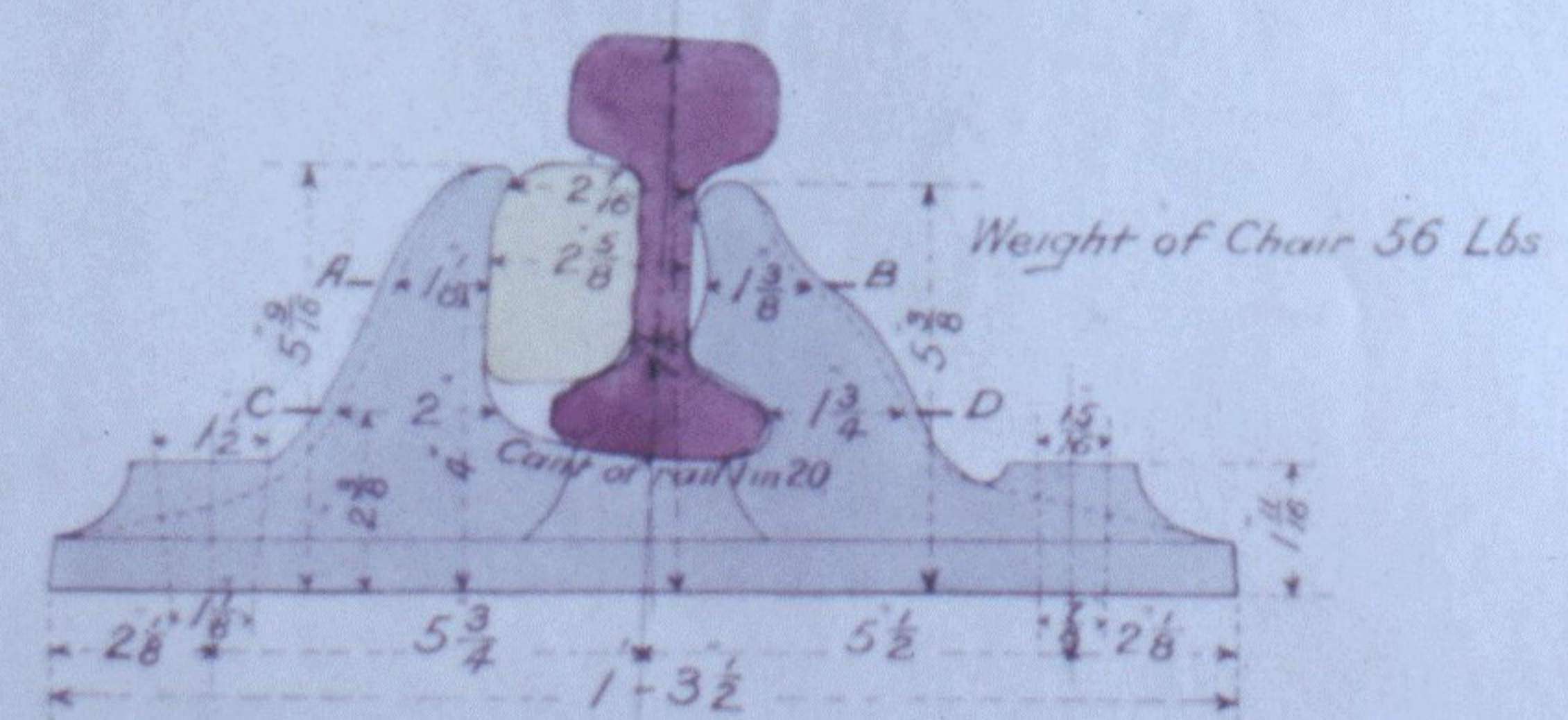
ELEVATION OF CHAIR
