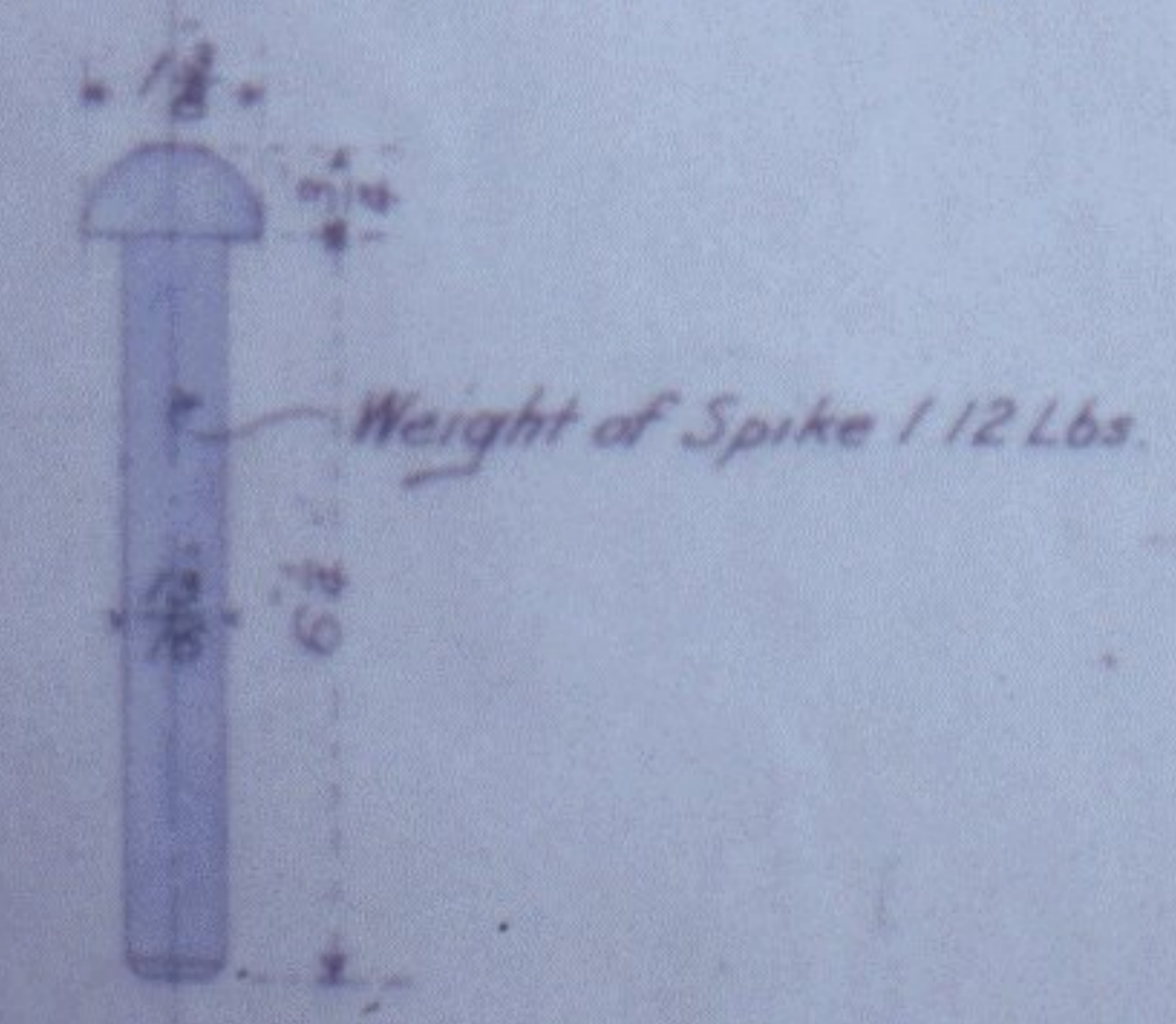
WROUGHT IRON SPIKE
