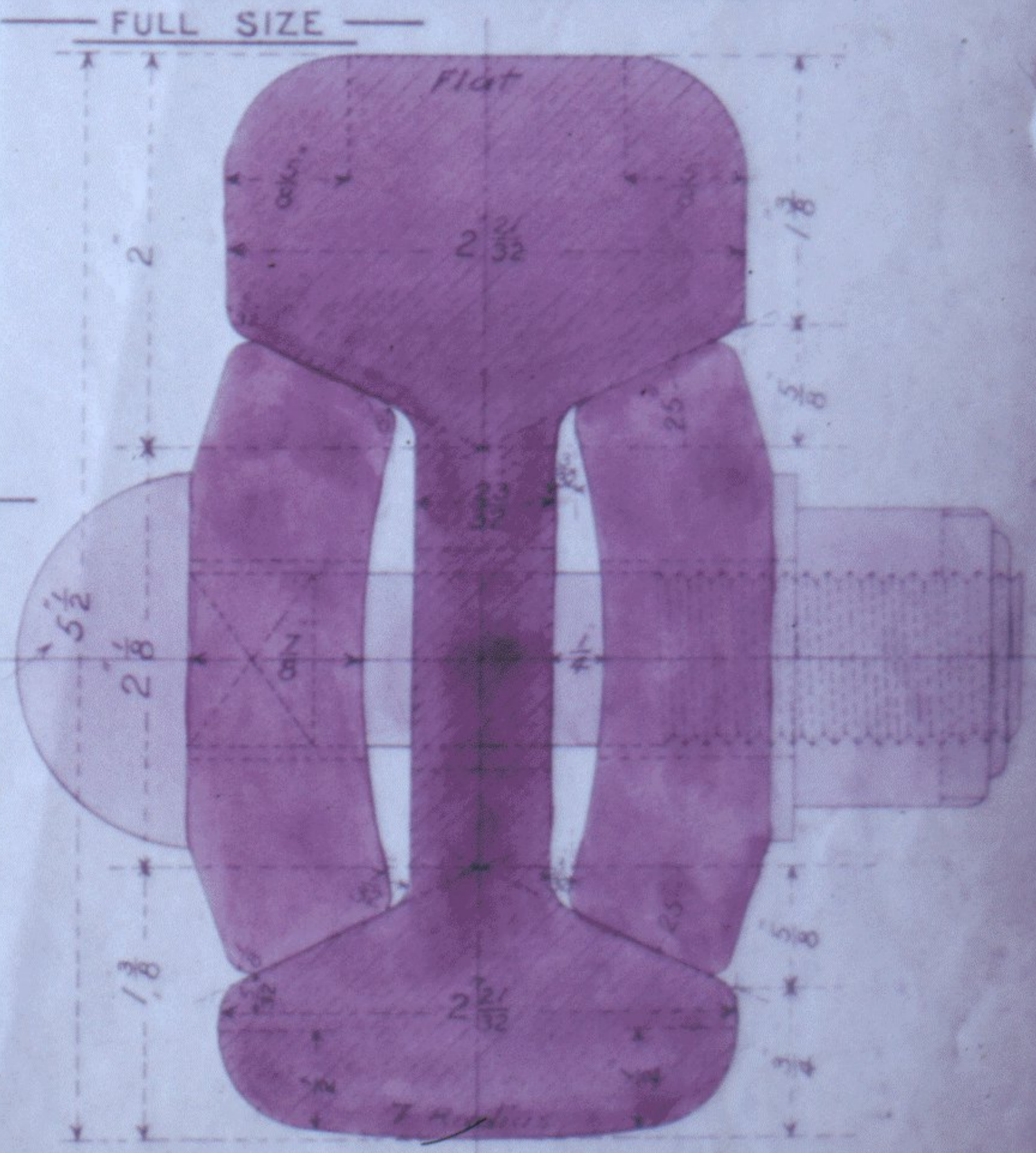
BOLT HOLE THROUGH FISH-PLATES — BOLT HOLE THROUGH RAIL
