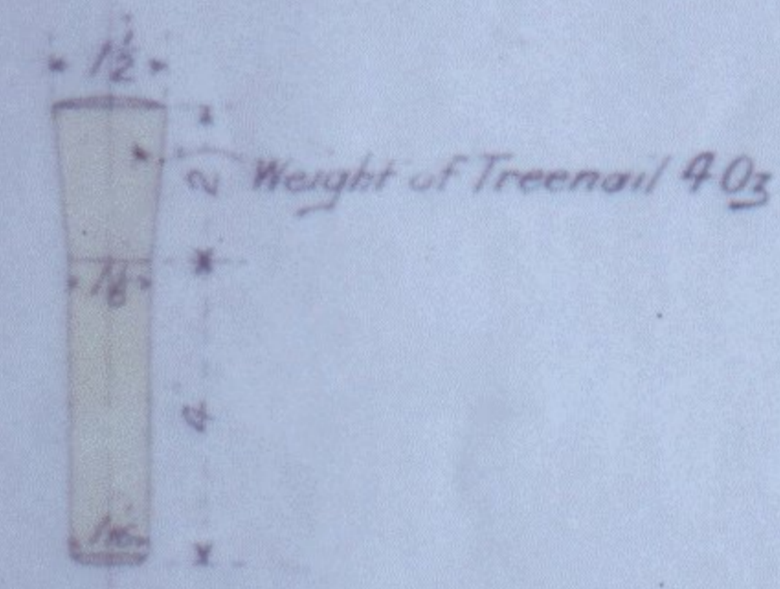
ENGLISH OAK PRESSED TREENAIL
