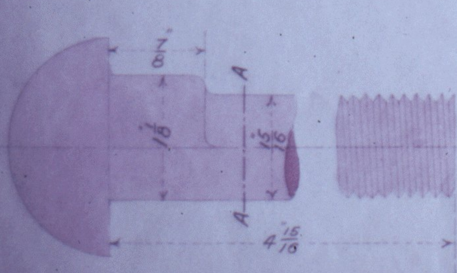
DETAIL SHEWING LUG ON BOLT.
