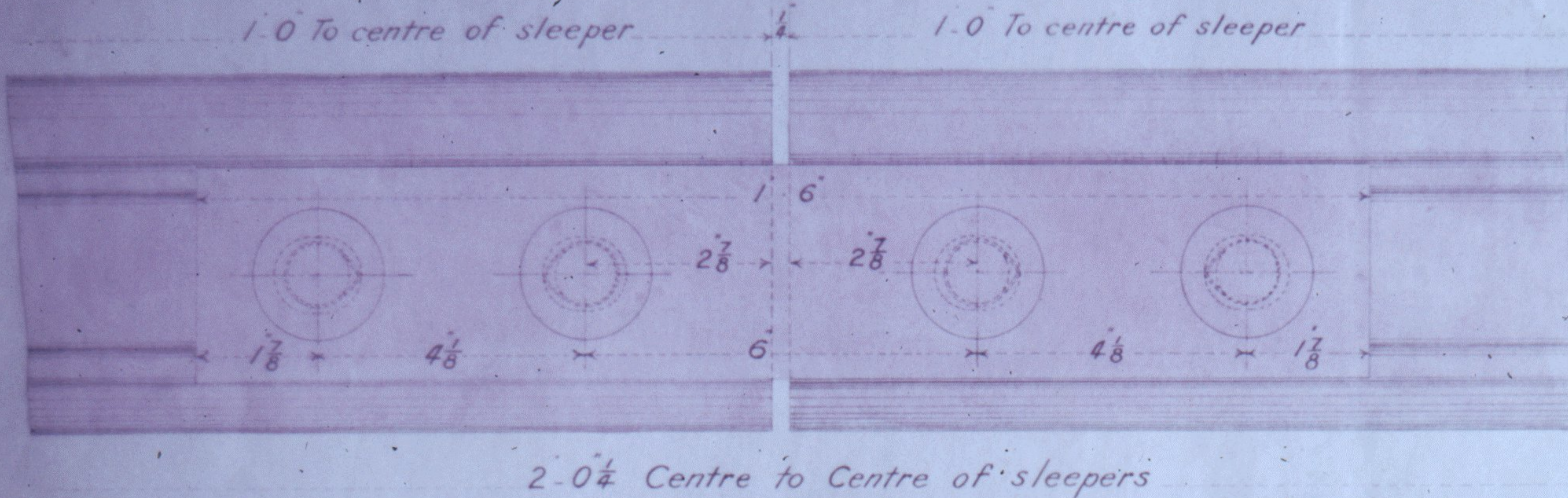
ELEVATION OF JOINT SHEWING FISH-PLATE
