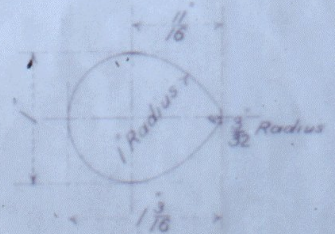
BOLT HOLE THROUGH FISH-PLATES.
