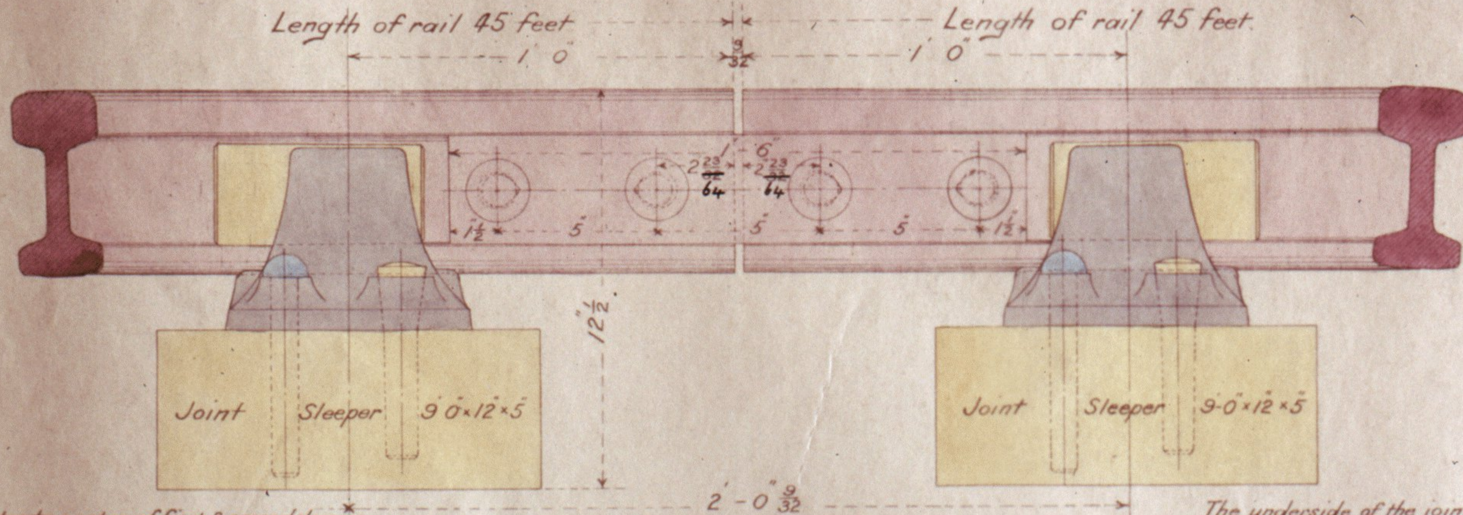
ELEVATION OF JOINT SHEWING FISH-PLATE.
