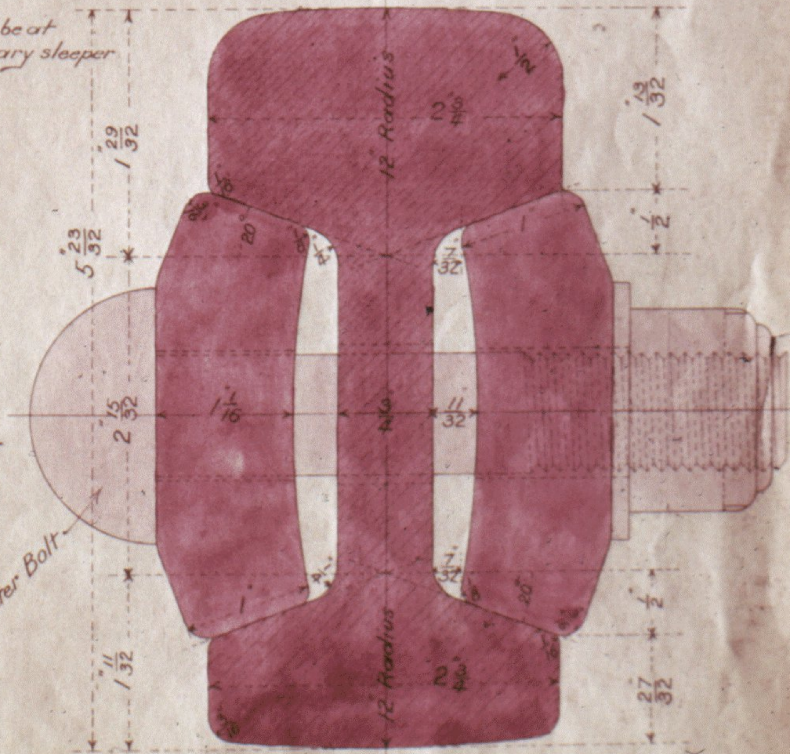
TO BE MADE RIGHT AND LEFT HAND.
