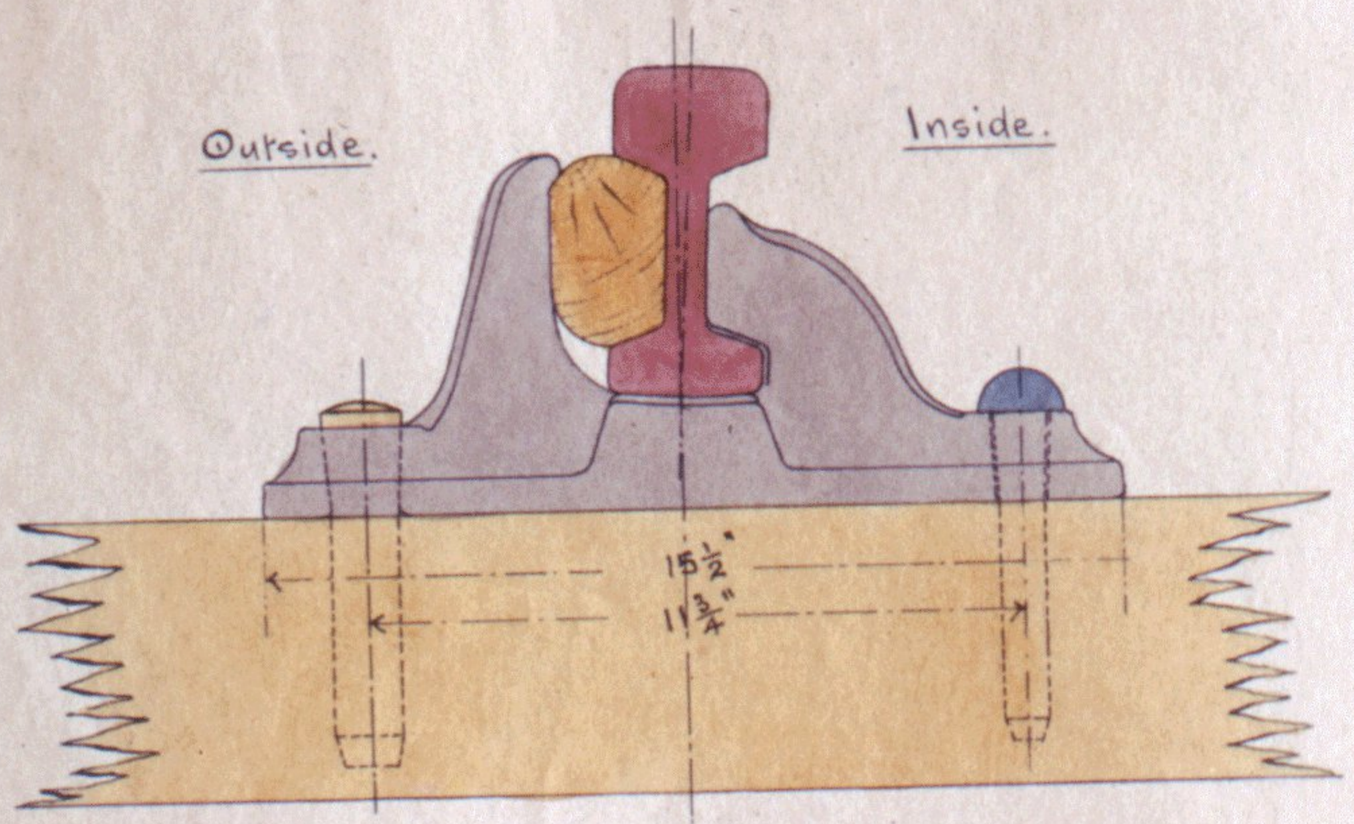
ELEVATION.
