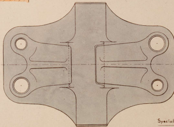
— PLAN OF SPECIAL CHAIR. —
