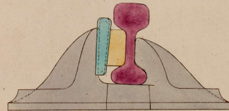
— ELEVATION WITH AUTON'S KEY. —
