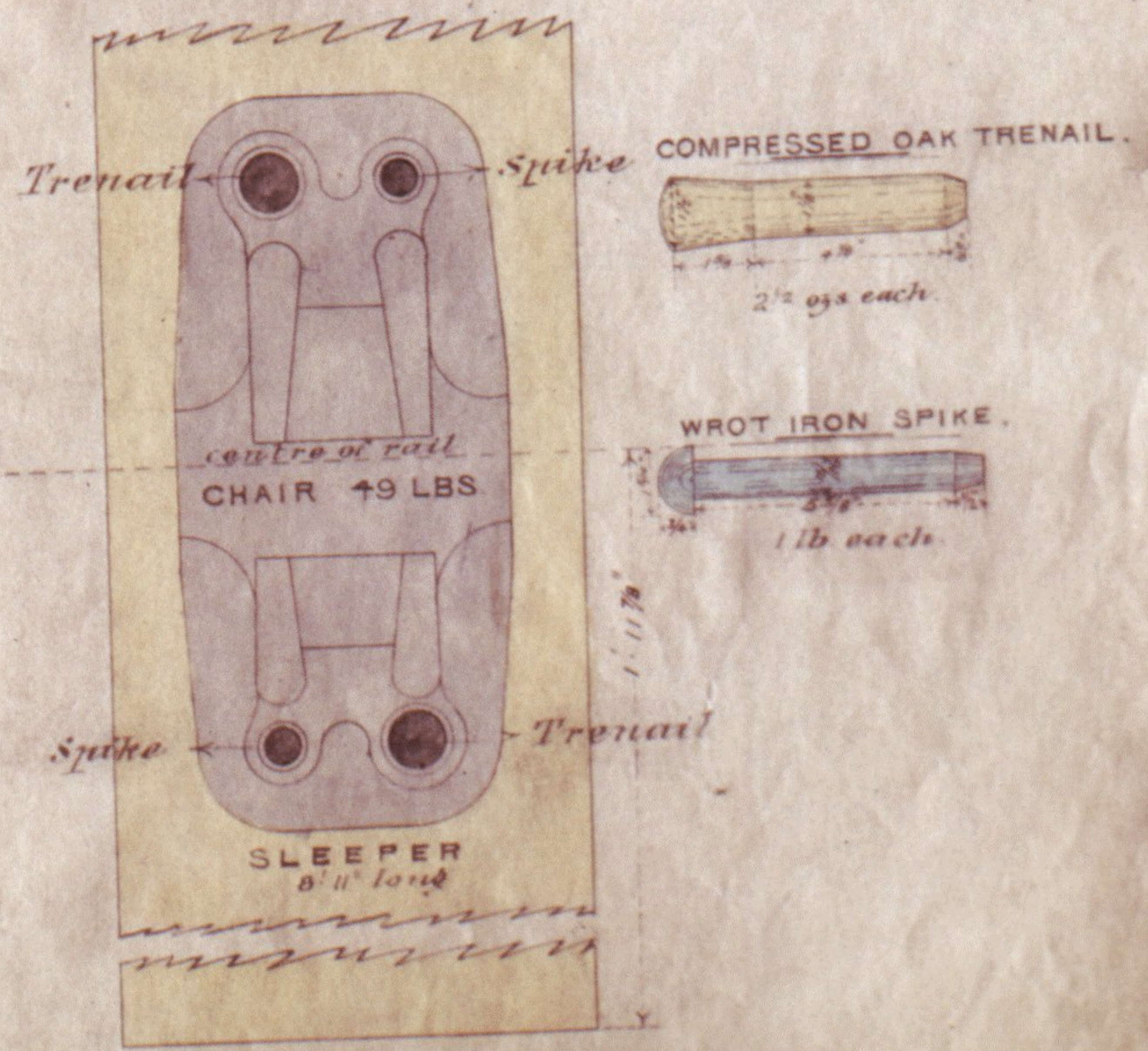
PLAN SHOWING CHAIR ON SLEEPER.
