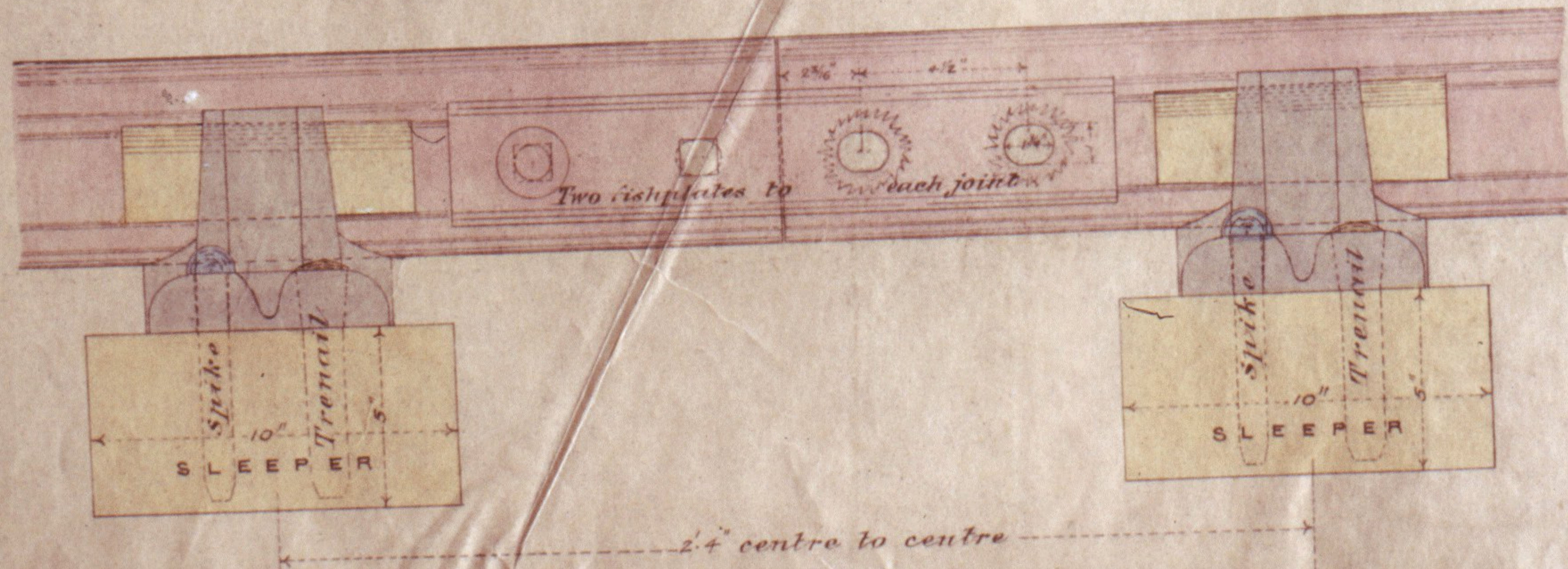
ELEVATION OF JOINT SHOWING SLEEPER ON EACH SIDE.
