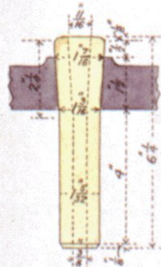
TREENAIL
