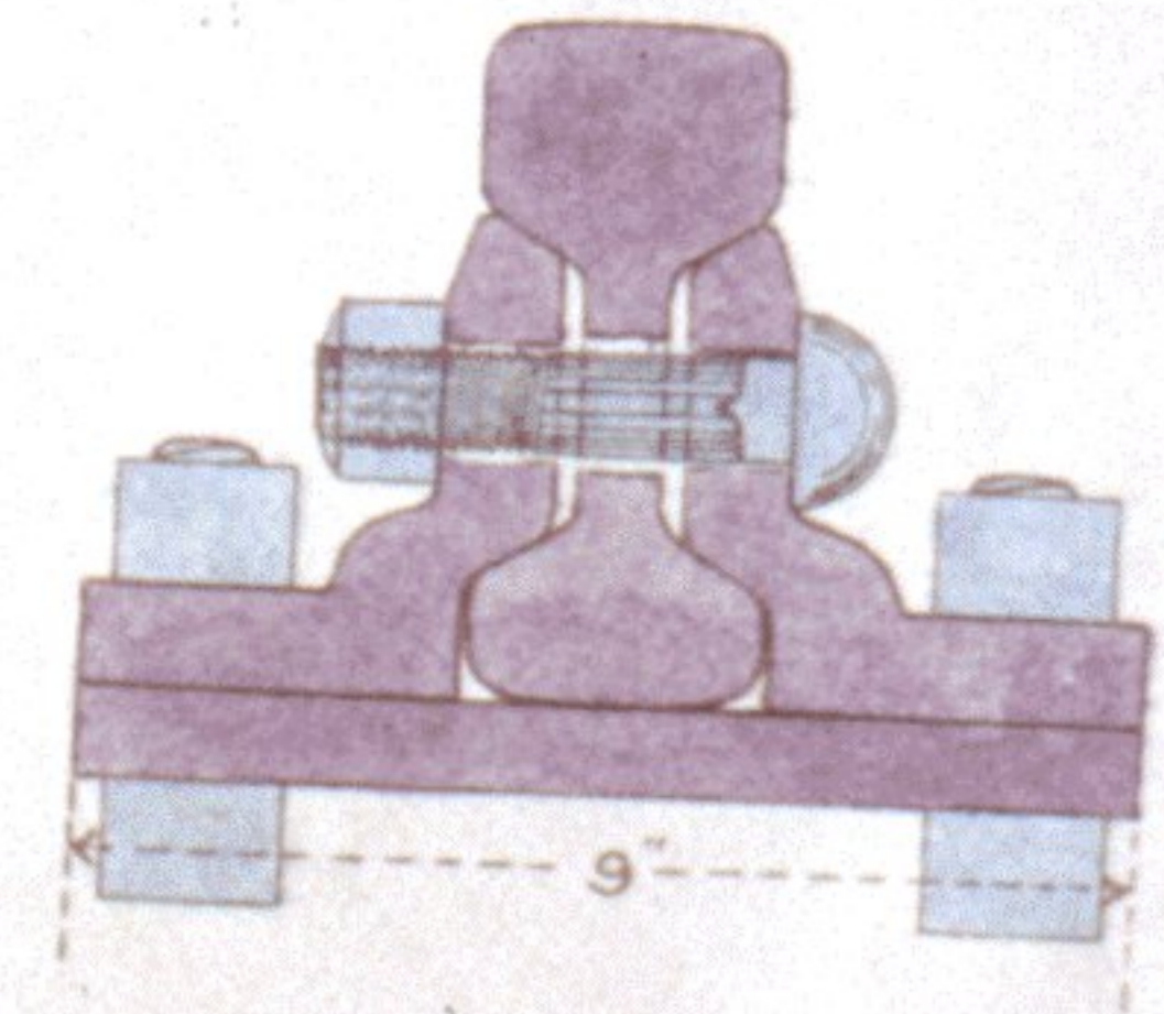
CROSS SECTION
