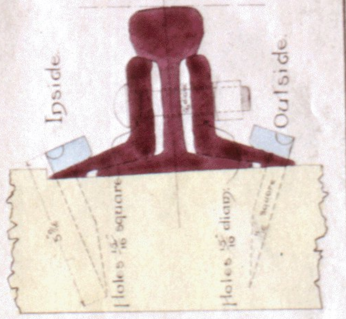
CROSS SECTION
