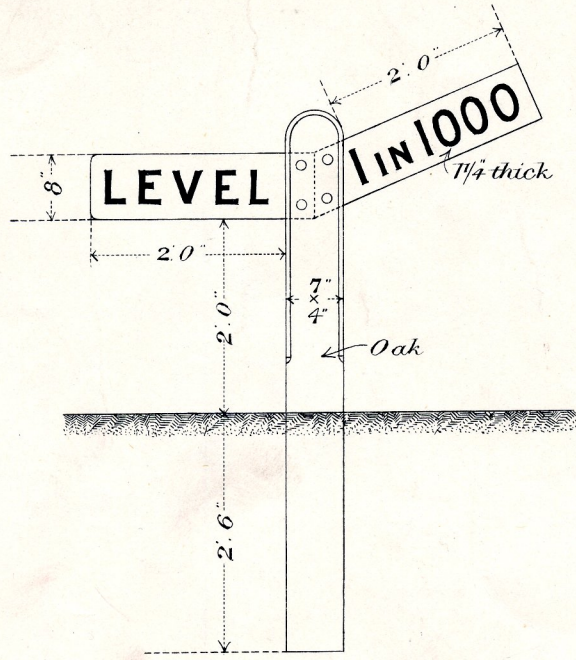
GRADIENT BOARD.
