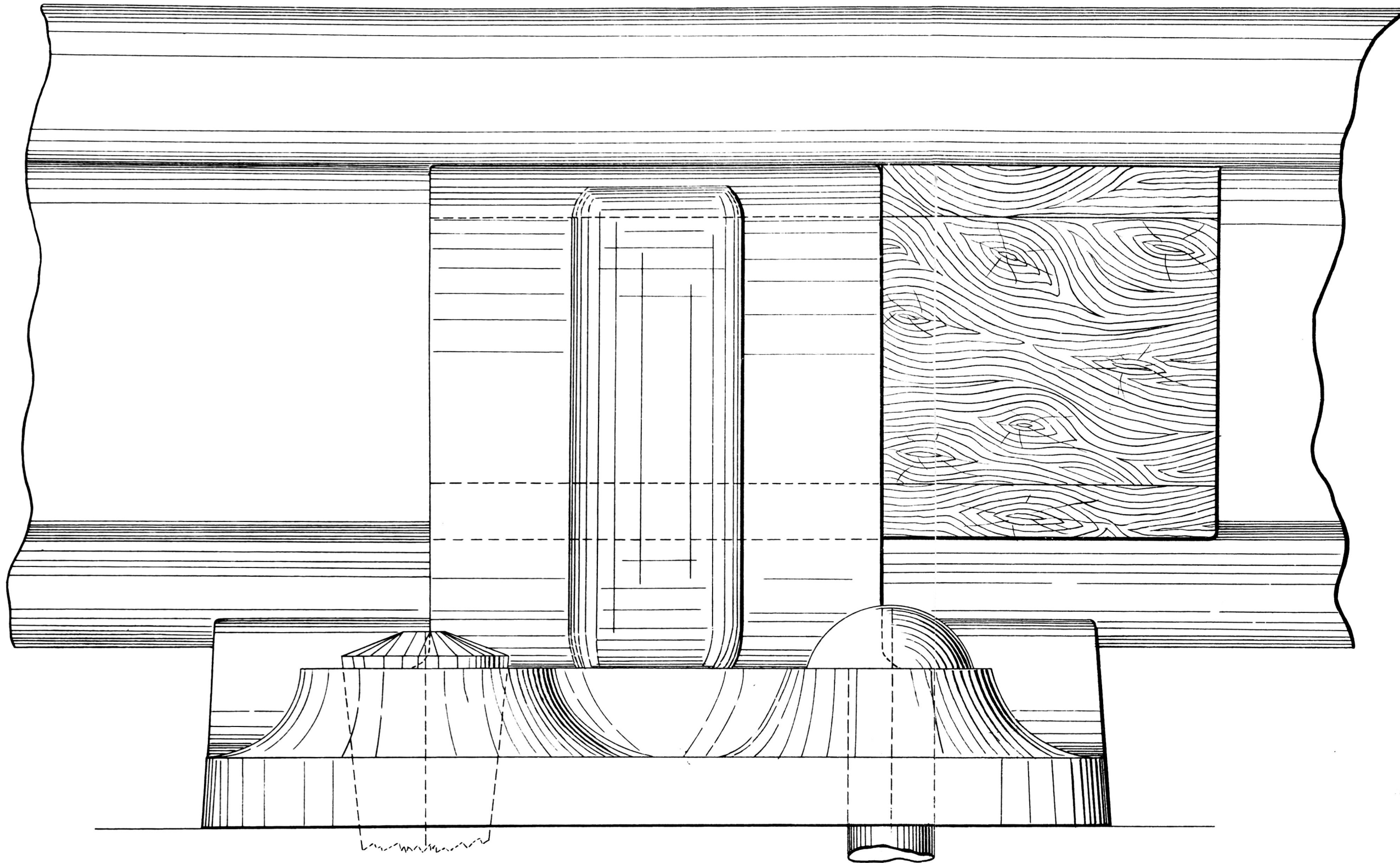
END ELEVATION.
