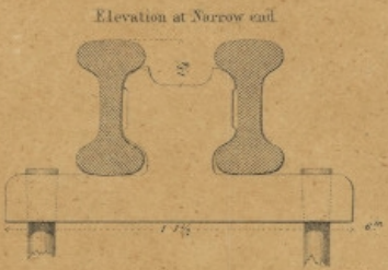
Elevation at Narrow end.
