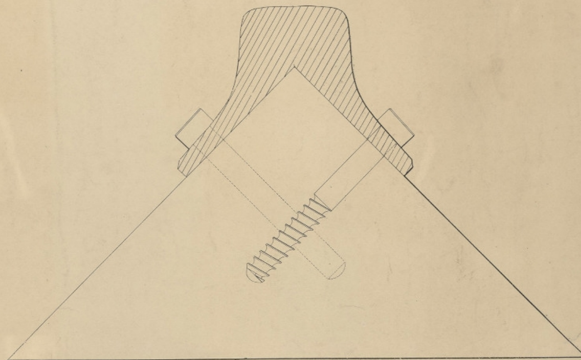
FIG. 4. FISH PLATE UNDER RAIL-JOINT.
