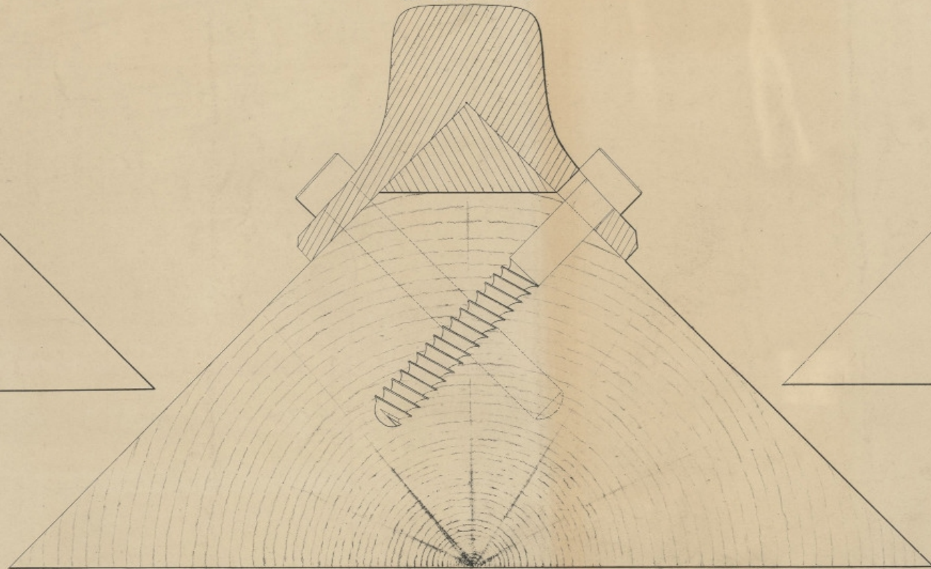
FIG. 1. 60 LBS. P r YARD
