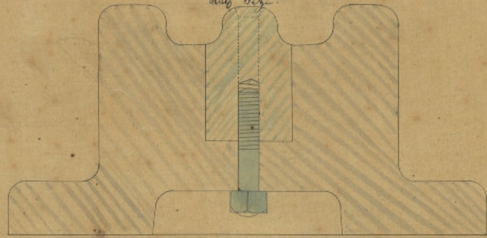
Ransomes & Biddells Patent Solid Chilled Crossing.
