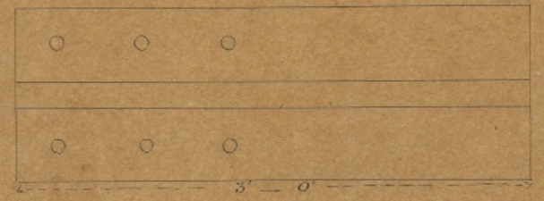
Plan of Joint Plate Fig 5
